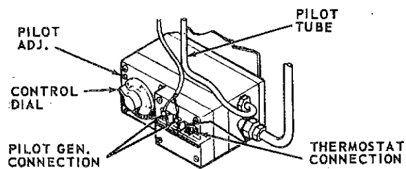
MILLIVOLT CONTROL
